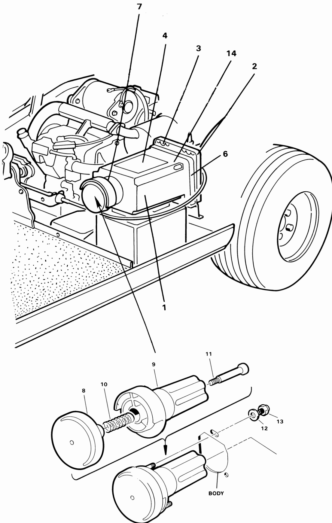
EXPANSION CHAMBER, CHOKE AND FILTER
