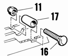
DETAIL E
