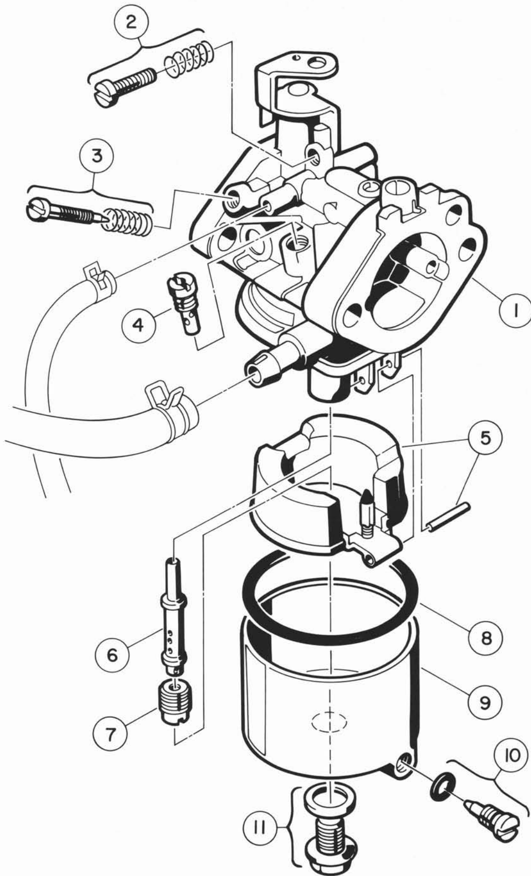
CARBURETOR ASSEMBLY
