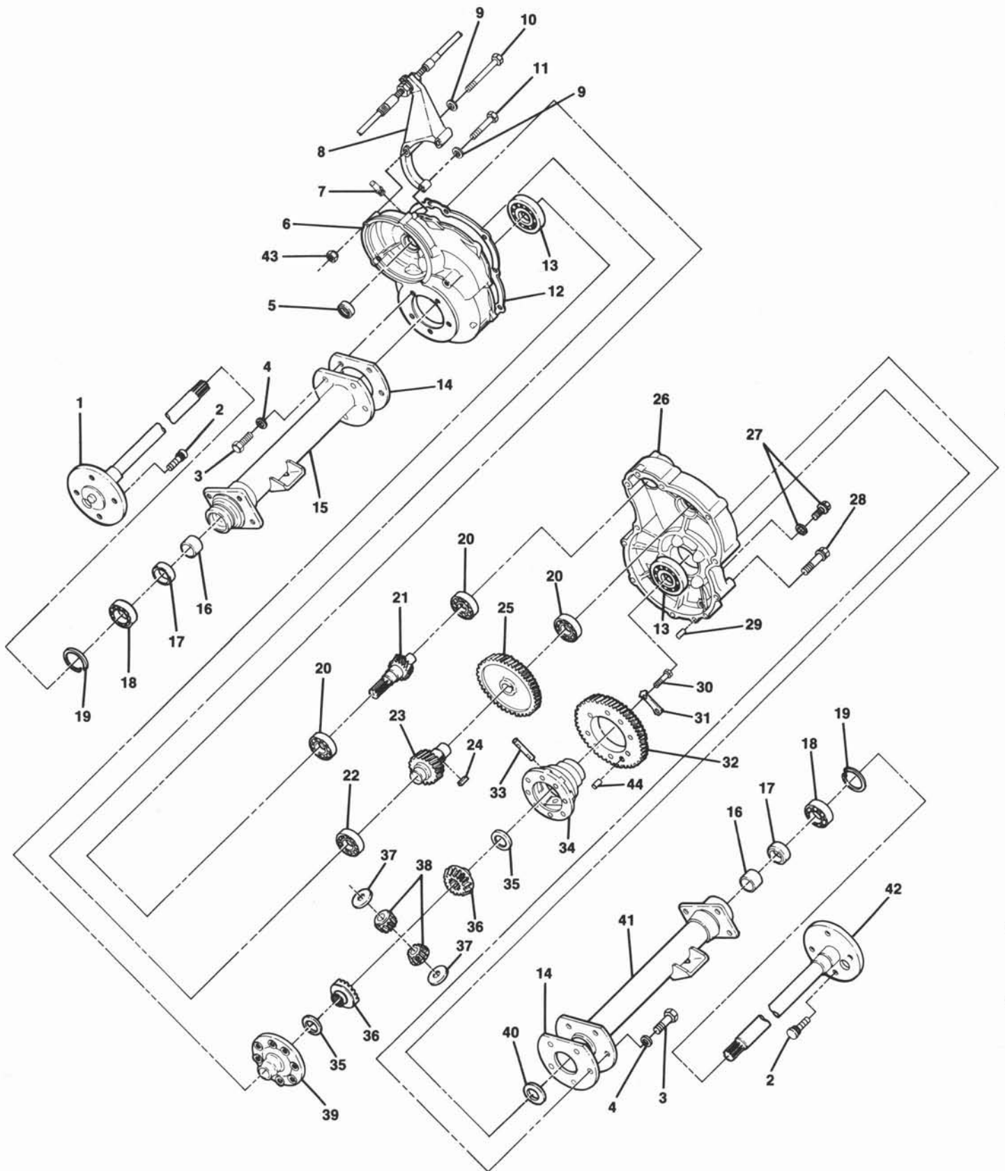
TRANSAXLE
